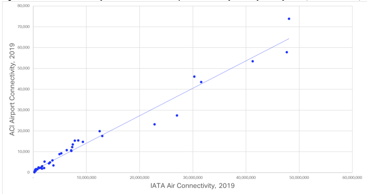
Figure 6a: IATA's air connectivity score and NetScan's airport connectivity score by country, 2019 (correlation=0.98)
